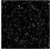
Gauss- Elimination
