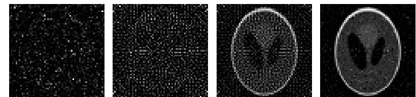
Gauss-Elimination
