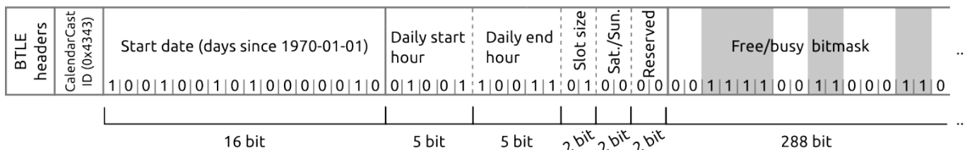
Figure 2. Bit-level description of CalendarCast message format (all numbers represented in network byte order, i.e. big endian format as suggested by [14]). This message is split and encapsulated in two BTLE broadcast frames.
