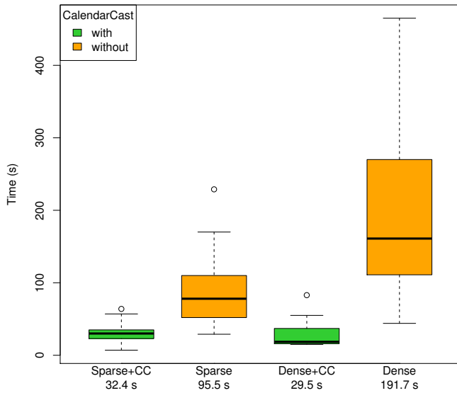
Figure 3. Task performance (boxes show 2nd and 3rd quartile, with median highlighted). Mean value is indicated below each condition.
