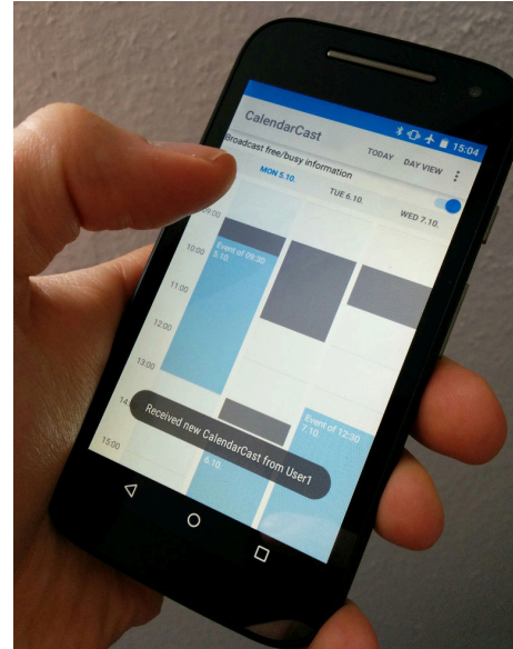
Figure 1. CalendarCast user interface. Own calendar entries are shown colored, while received broadcasts are shown as anonymous grey events in the background. Reception of a new broadcast is indicated by a popup message.
