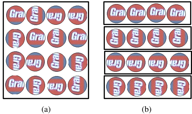
Figure 3. Examples of patches used for classification. (a) To estimate the keypoint identity, patches from the same keypoint are grouped in a single class. (b) To estimate the patch transformation, several classes for different transformations are created for each keypoint in the database.
