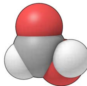
Fig. 2 Space Filling Model
