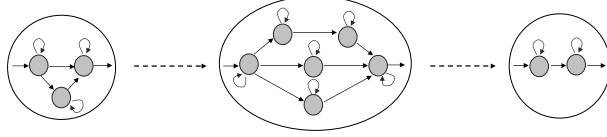
Figure 6: A-priori phase-wise model construction: Sub-HMMs are constructed for each phase or cluster of data and appended as displayed in this image.
