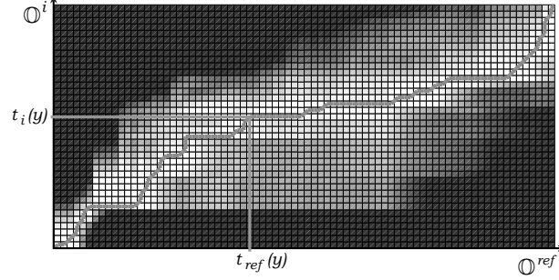
Figure 3: DTW distance matrix. The path drawn through the valley displays the optimal synchronization between surgeries \mathbb{O}^i and \mathbb{O}^{ref} .
