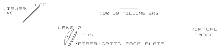
Fig. 2. The layout of our HOE-based autostereoscopic in-situ visualization system.
