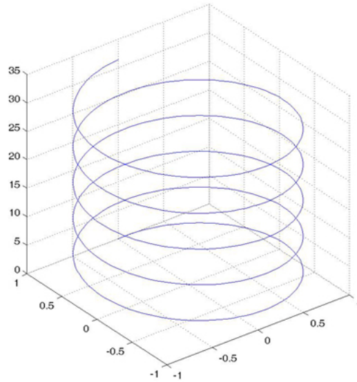
Figure 3: 3D Plot
