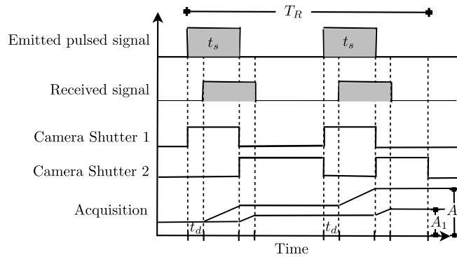
Figure 3.2.: Pulse wave time-of-flight camera working diagram. [80]
