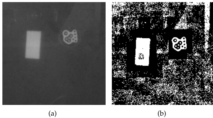
Figure 4.33.: Berensen threshold. (a) The source monochrome image; (b) The binarized image after performing a Berensen threshold.
