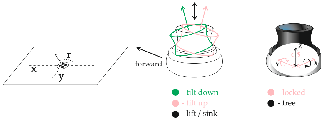
Figure 4.34.: Fiduciary marker and 3D mouse used for camera control. Left: 2D position and orientation (x, y and r) of the camera is determined by the fiduciary marker on the table surface; Middle: permitted directions of movement of the 3D mouse to control the camera; Right: free and locked axes of the 3D mouse controller.
