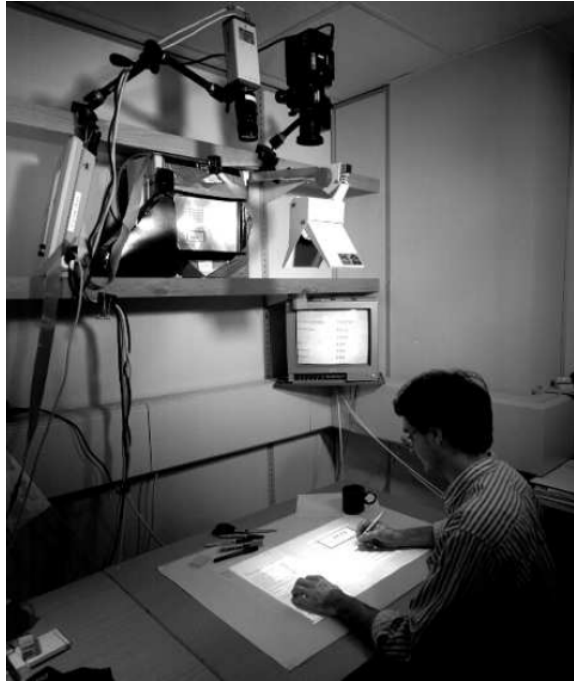
Figure 2.1.: DigitalDesk [9]
