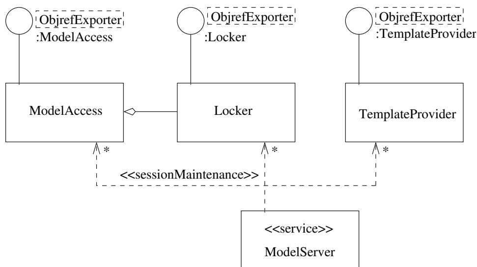
Figure 7.11: UML-diagram: The ModelServer's arrangement of classes
