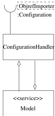
Figure 7.13: UML-diagram: The interface of the Model service to access its configuration
