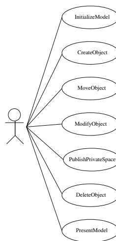
Figure 3.2: UseCases
