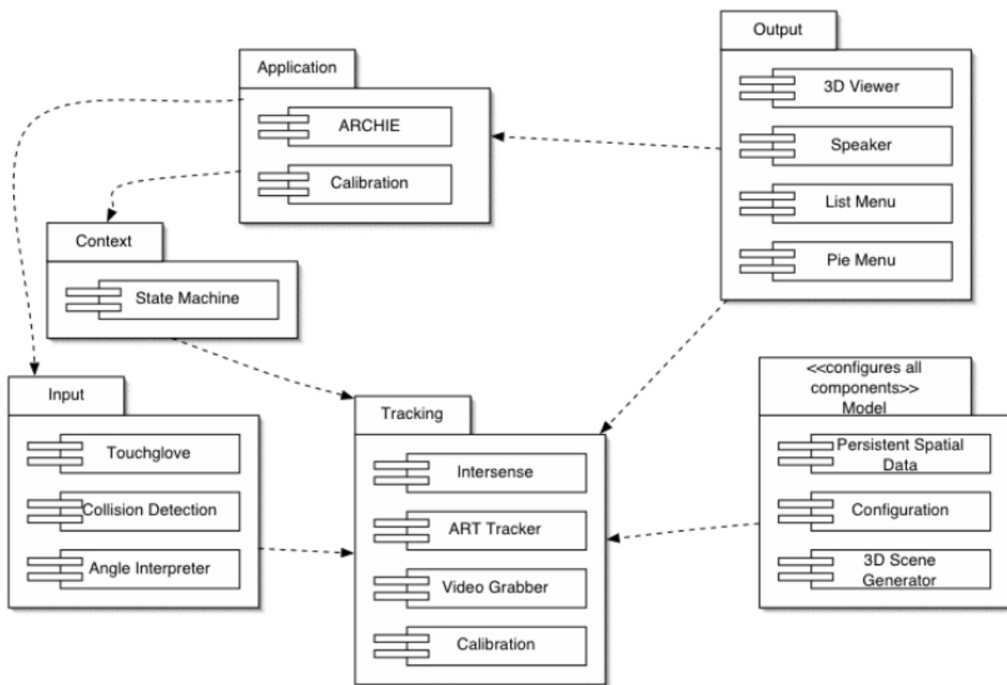
Figure 2.11: ARCHIE architecture
